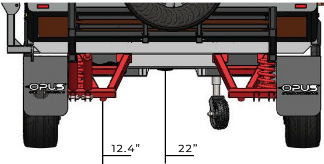
GROUND CLEARANCE
