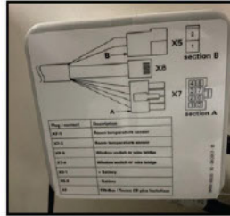
Junction Box
