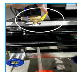
DRAIN VALVE- OPEN POSITION FIGURE B2
