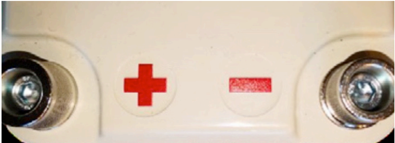
FIGURE 3. DIFFERENCE DIAMETER OF + AND - POLE
